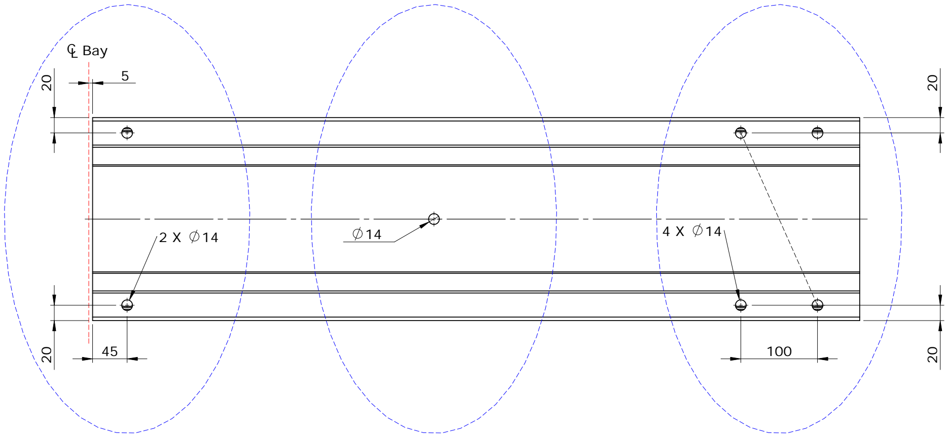
TYPICAL END CLEAT PUNCHING ARRANGEMENT
