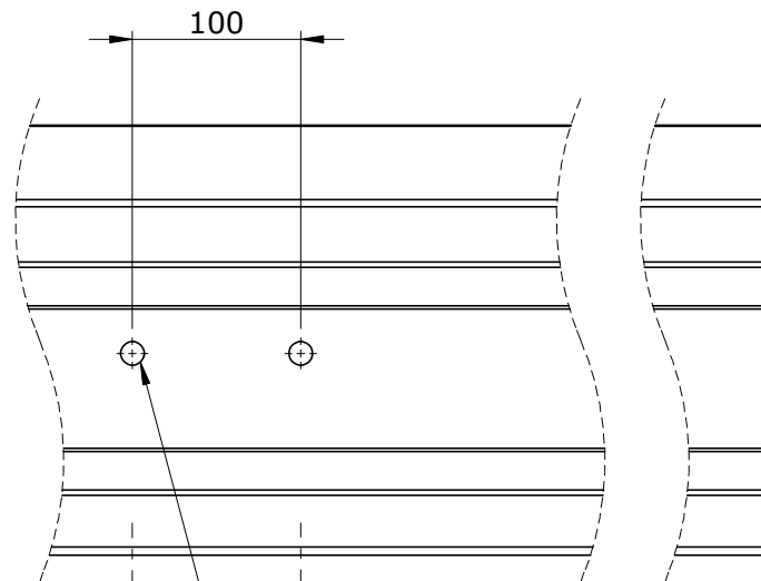
EAVES STRUT CLEAT HOLES - 4 X 14MM
